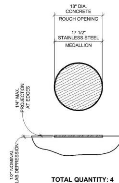
TYPICAL BELVEDERE MEDALLION
