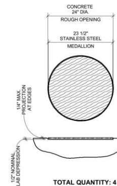
TYPICAL LANDING MEDALLION
