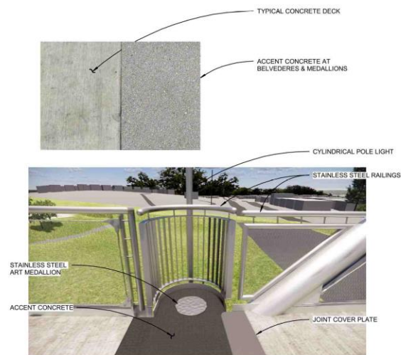
ART MEDALLION CONTEXT RENDERING (BENT 4)
