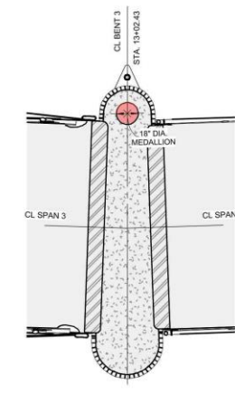
4: BELVEDERE MEDALLION PLAN AT BENT 3
