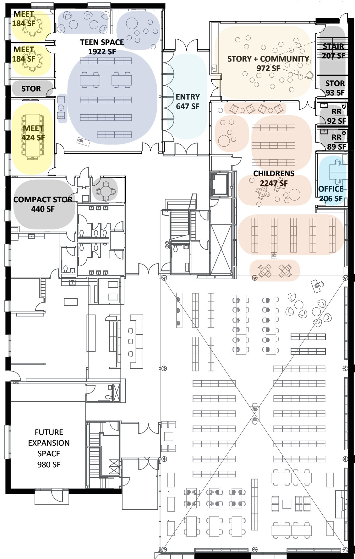
LEVEL 01
