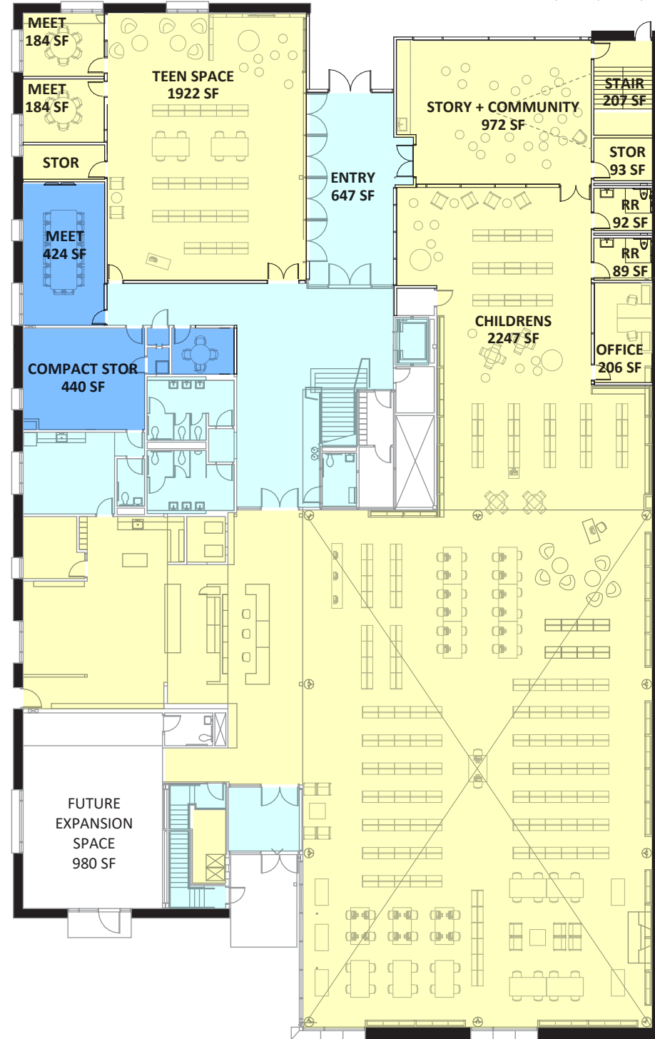
LEVEL 01
